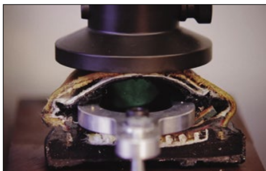
Toe Cap Compression Testing
