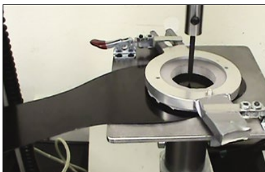
Puncture Resistant Testing
