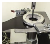
Above: The steel pin is forced into the midsole to determine the amount of force required to puncture the material.
